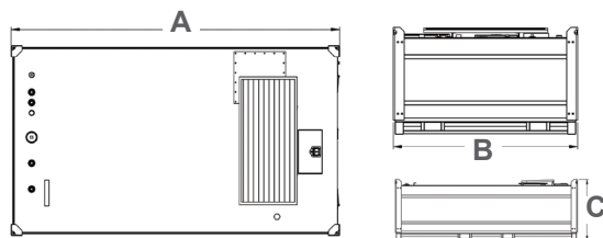
Cubes Dimensions
